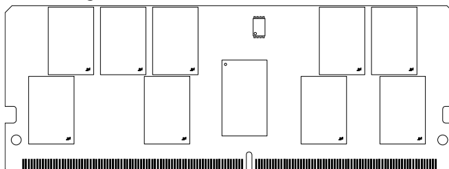
Figure 1: 288-Pin MiniRDIMM (MO-314, R/C-ZZ)
