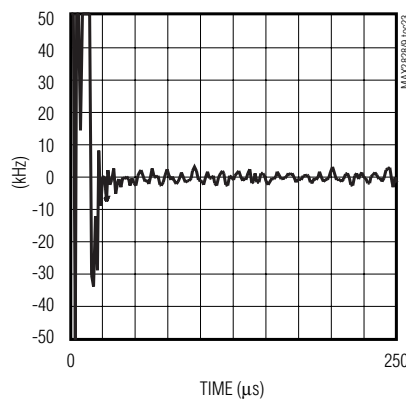
CHANNEL-SWITCHING FREQUENCY SETTLING (2500MHz TO 2400MHz)
