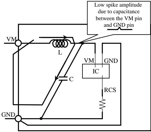
Figure 3. Recommended pattern
