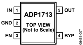
Figure 7. 5-Lead TSOT (UJ-Suffix)
