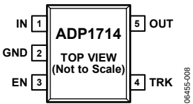
Figure 8. 5-Lead TSOT (UJ-Suffix)
