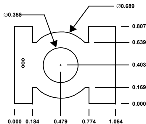
Figure 15. PWB Dimensions
