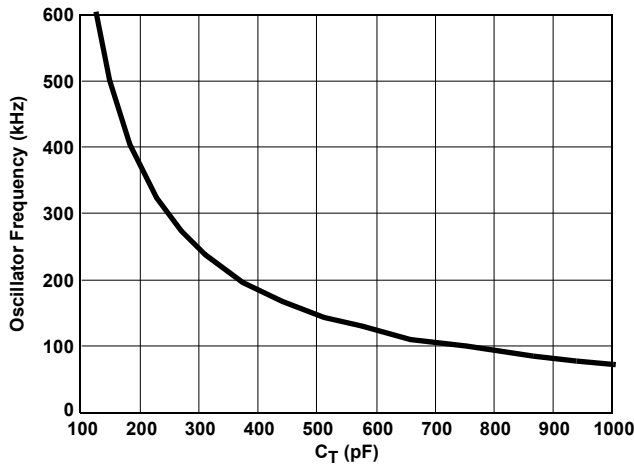
Figure 5. Capacitance vs Oscillator Frequency ( R_{TD} = 49.9k\Omega )
