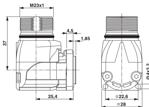
Dimensional drawing
