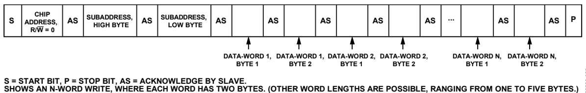
Figure 23. Burst Mode I 2 C Write Format
