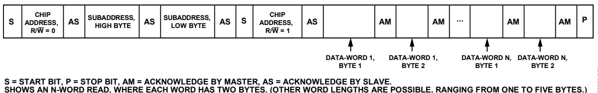
Figure 25. Burst Mode I 2 C Read Format
