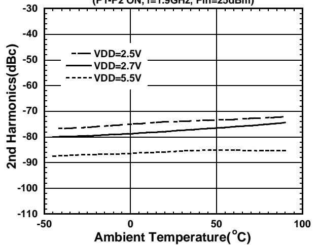
2nd Harmonics vs. Ambient Temperature
