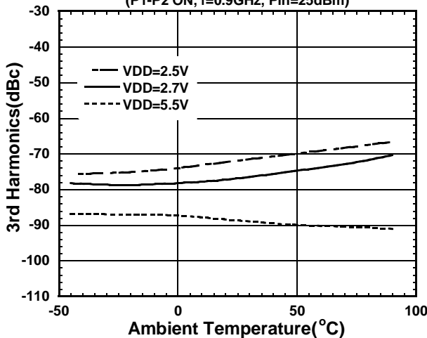
3rd Harmonics vs. Ambient Temperature
