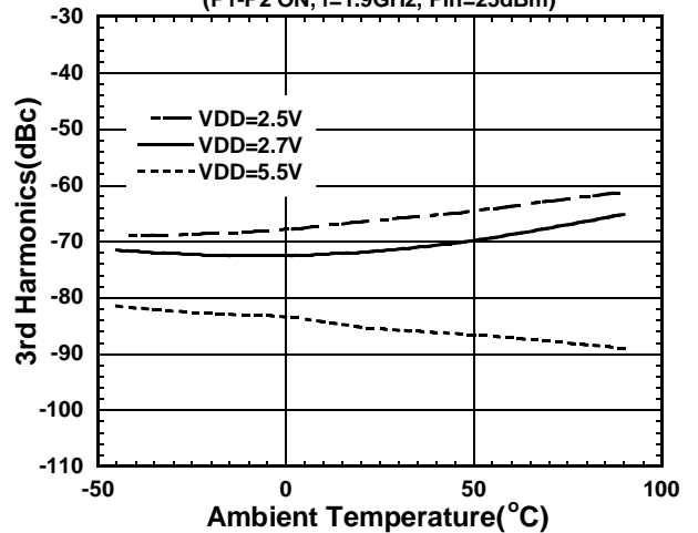
3rd Harmonics vs. Ambient Temperature
