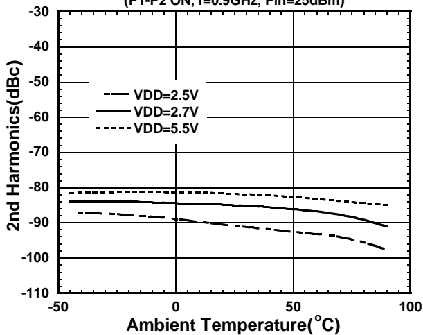
2nd Harmonics vs. Ambient Temperature
