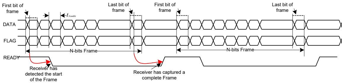
Figure 73. Receiver Real-Time Data Flow READY Signal Timing
