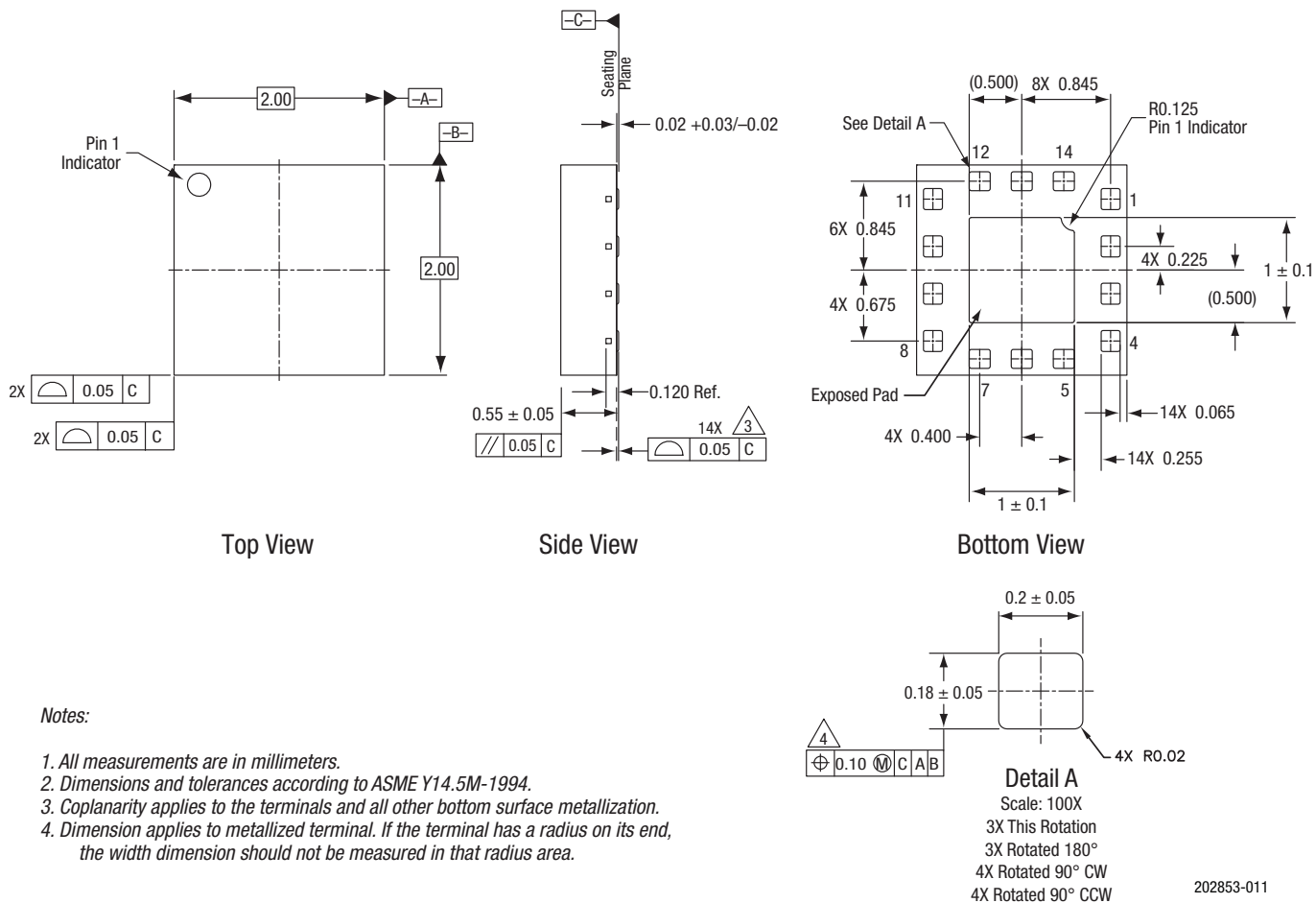
Figure 11. SKY13526-485LF Package Dimensions
