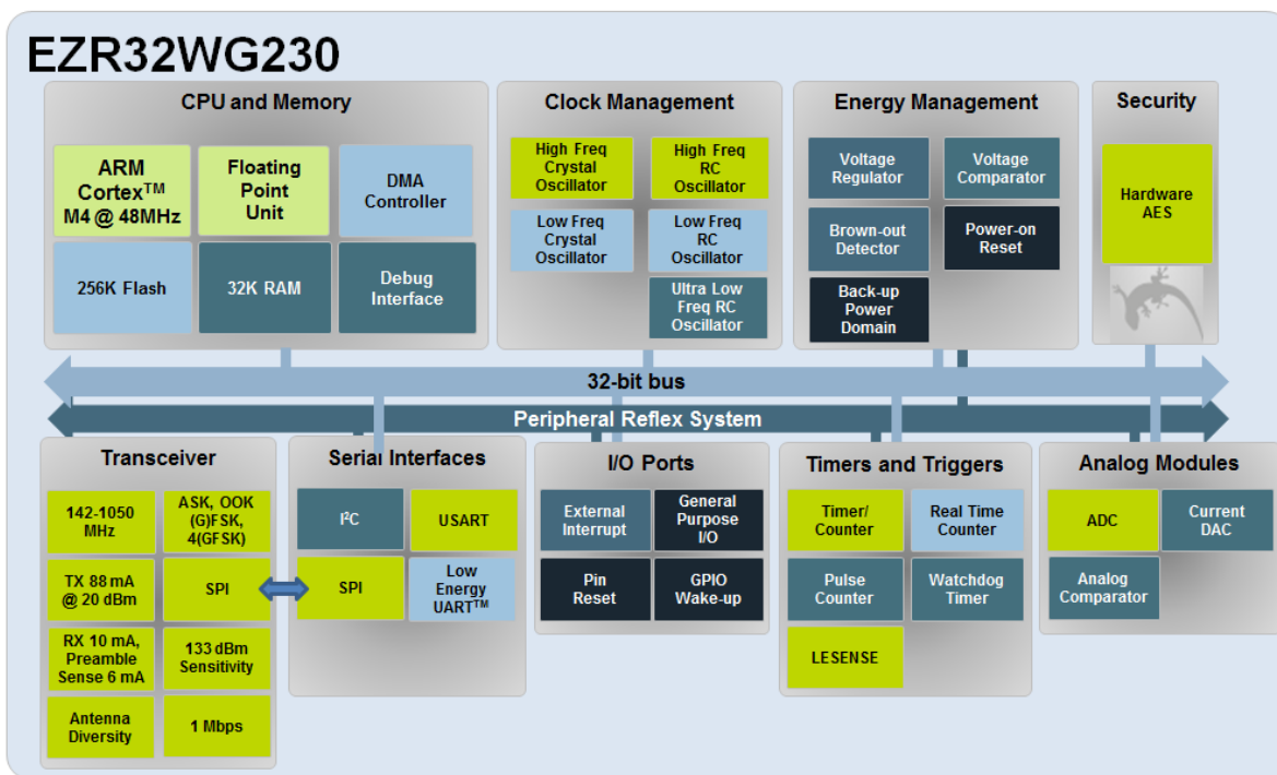
Figure 3.1. Block Diagram
