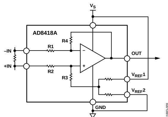
Figure 32. Split Supply
