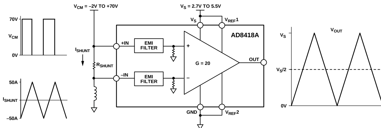
Figure 28. Typical Application
