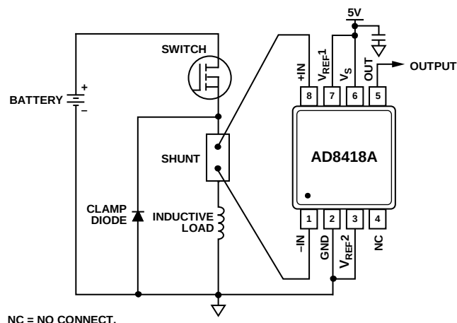
Figure 37. High-Side Switch
