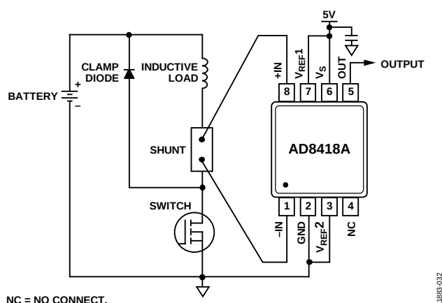
Figure 36. Low-Side Switch
