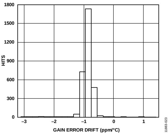
Figure 27. Gain Error Drift Distribution
