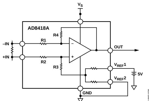
Figure 33. Split External Reference
