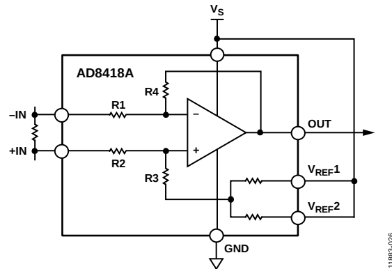
Figure 30. V_S Referenced Output
