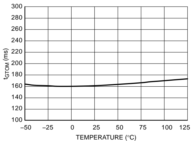
Figure 42. Go To Off Mode Timer Duration t_{GTOM}
