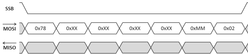
Figure 25: Sequence of instructions to WRITE '0xFFFFFFFF' to address '0xMM' of the system registers
