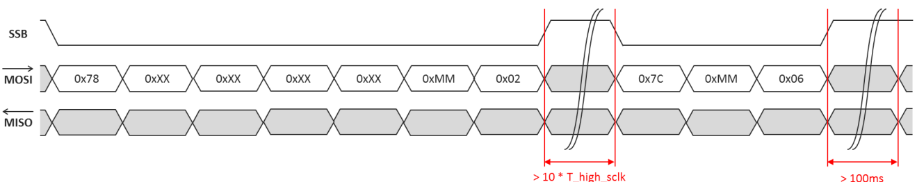
Figure 27: Sequence of instructions to WRITE data '0xFFFFFFFF' to address '0xMM' of the MTP
