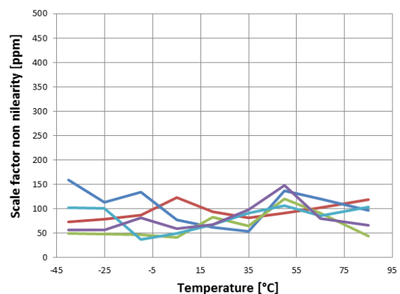
Figure 7 Scale factor non linearity over temperature (5 samples)
