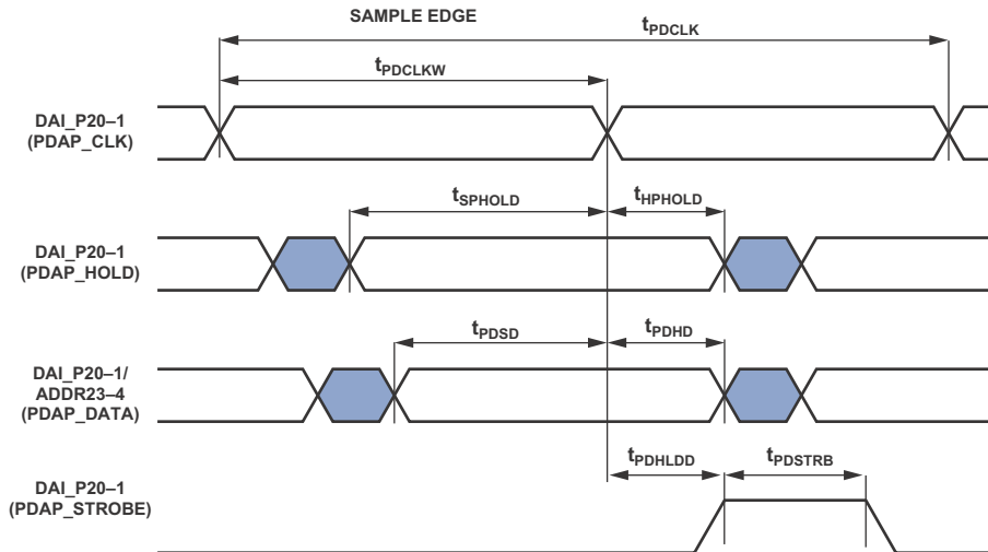
Figure 29. PDAP Timing
