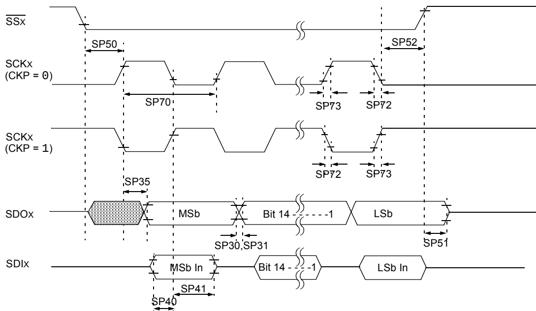
FIGURE 24-15: SPIx SLAVE MODE (FULL-DUPLEX CKE = 0, CKP = 1, SMP = 0) TIMING CHARACTERISTICS
