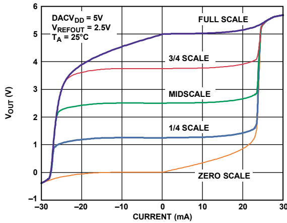
Figure 13. DAC Sink and Source Capability
