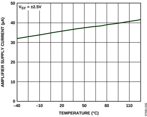
Figure 35. Amplifier Supply Current vs. Temperature
