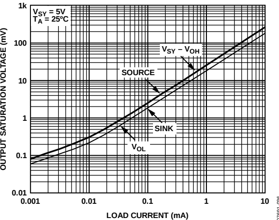
Figure 36. Amplifier Output Saturation Voltage vs. Load Current
