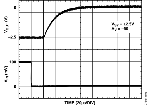
Figure 46. Amplifier Positive Overload Recovery
