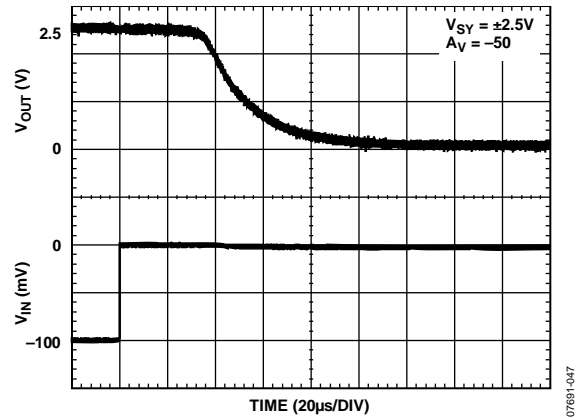
Figure 47. Amplifier Negative Overload Recovery
