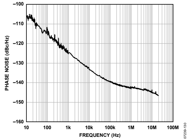
Figure 20. Additive (Residual) Phase Noise, CLK-to-LVPECL @ 1600 MHz, Divide-by-1
