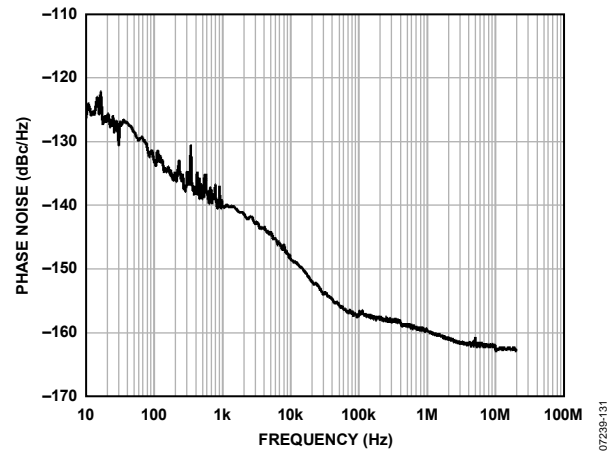
Figure 21. Additive (Residual) Phase Noise, CLK-to-CMOS @ 50 MHz, Divide-by-20
