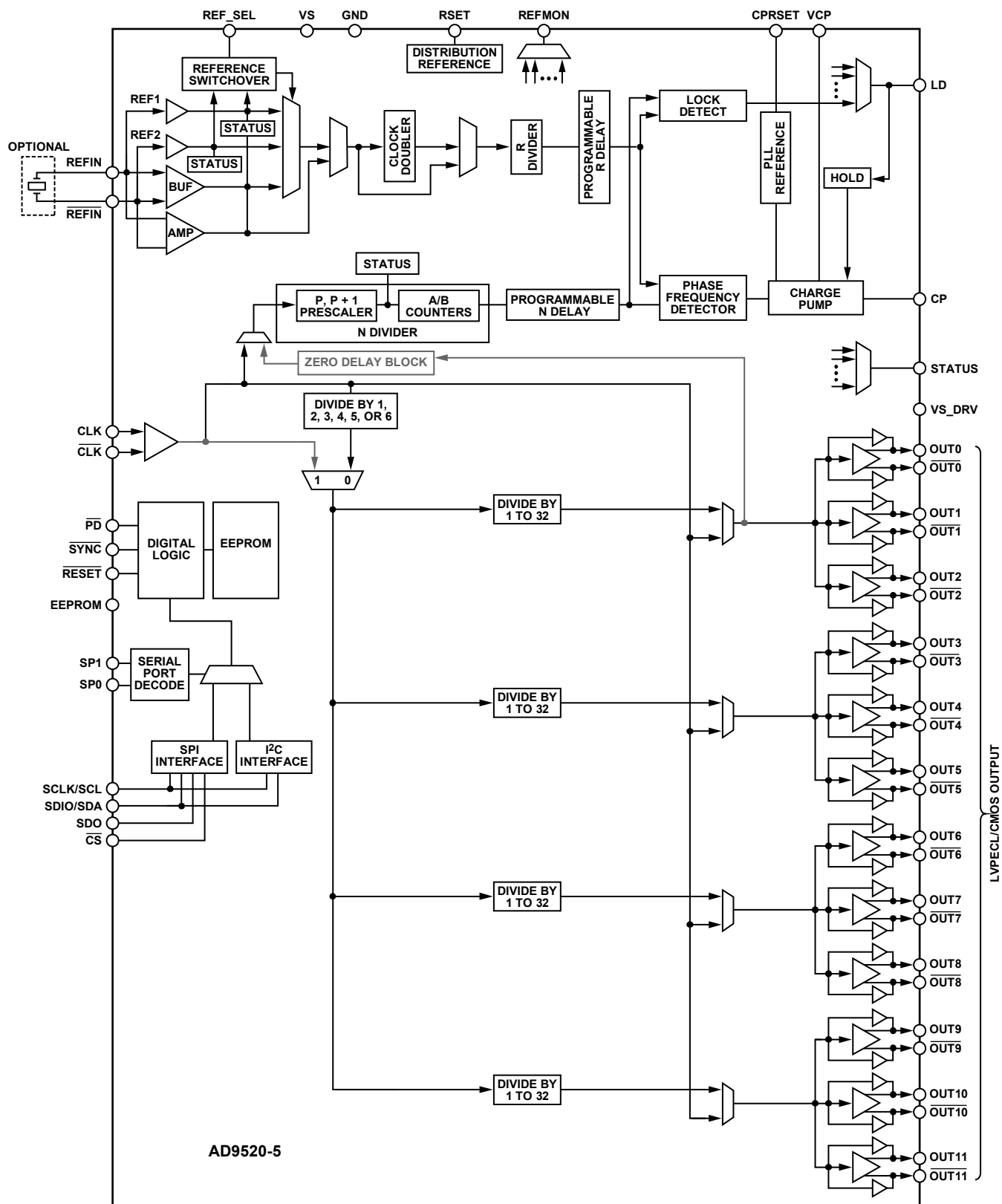
Figure 27. High Frequency Clock Distribution or External VCO &gt; 1600 MHz (Mode 2)
