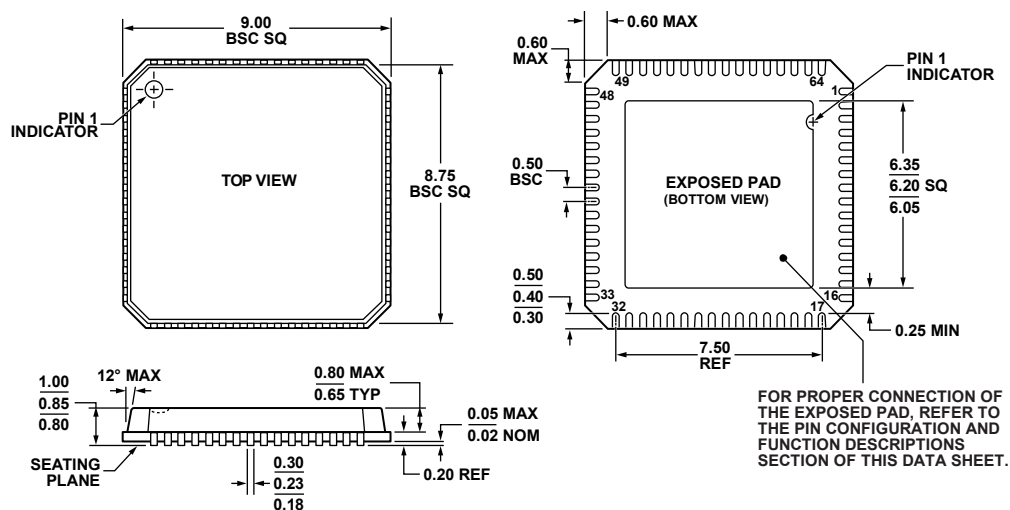
Figure 63. 64-Lead Lead Frame Chip Scale Package [LFCSP_VQ] 9 mm × 9 mm Body, Very Thin Quad CP-64-4
