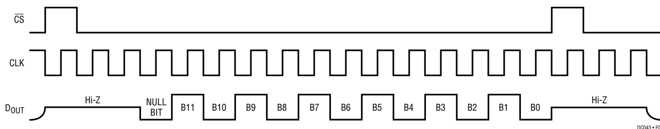
Figure 1. Timing Diagram
