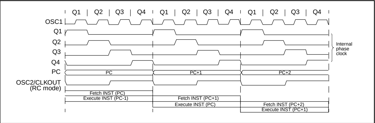
FIGURE 3-4: CLOCK/INSTRUCTION CYCLE
