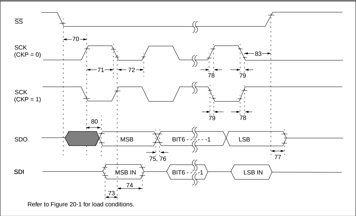
FIGURE 20-11: SPI SLAVE MODE TIMING (CKE = 0)
