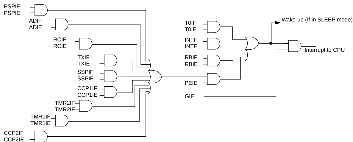
FIGURE 14-16: INTERRUPT LOGIC
