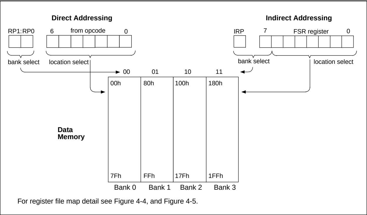
FIGURE 4-18: DIRECT/INDIRECT ADDRESSING
