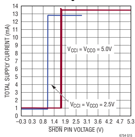
Total Supply Current vs SHDN Pin Voltage
