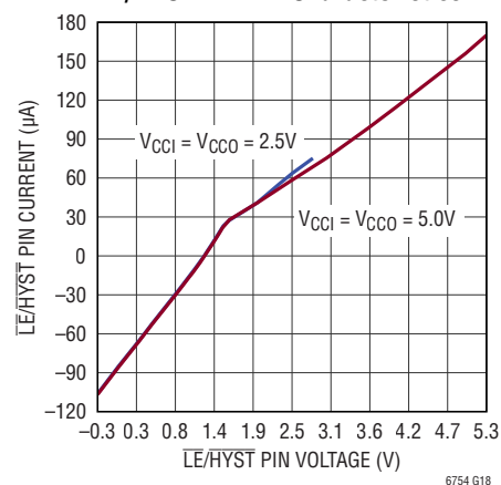
LE/HYST Pin I-V Characteristics
