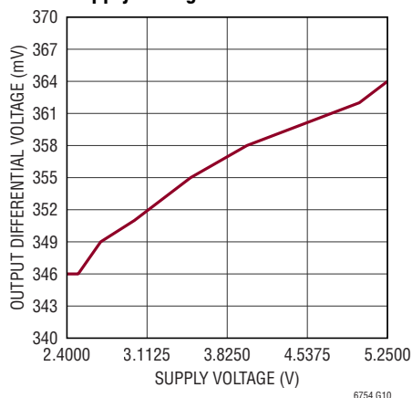
Output Differential Voltage vs Supply Voltage
