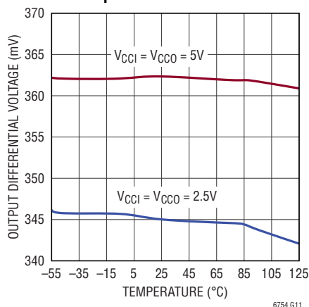
Output Differential Voltage vs Temperature
