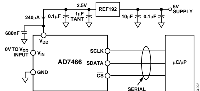
Figure 22. REF192 as Power Supply to AD7466
