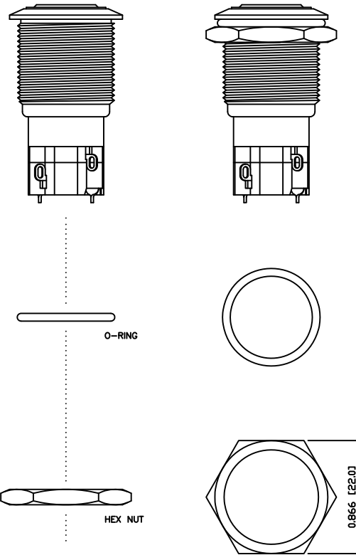
EXPLODED VIEW
