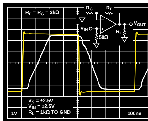
Figure 45. Overdrive Recovery
