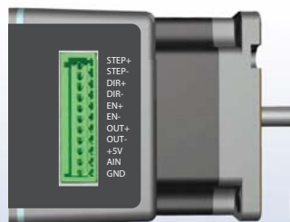
Input/Output connections
