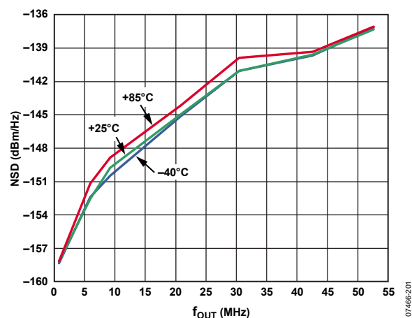
Figure 64. NSD at 8 mA, 1.8 V
