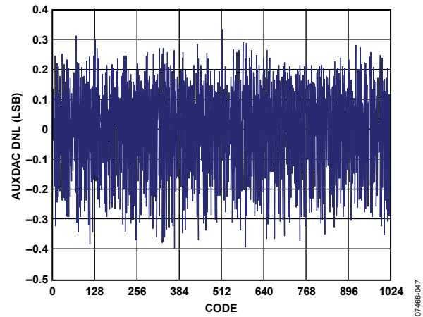
Figure 40. AUXDAC DNL
