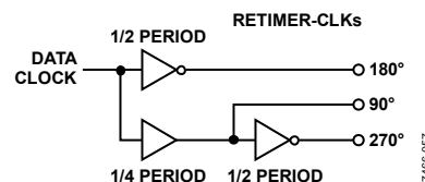
Figure 82. RETIMER-CLK Phases
