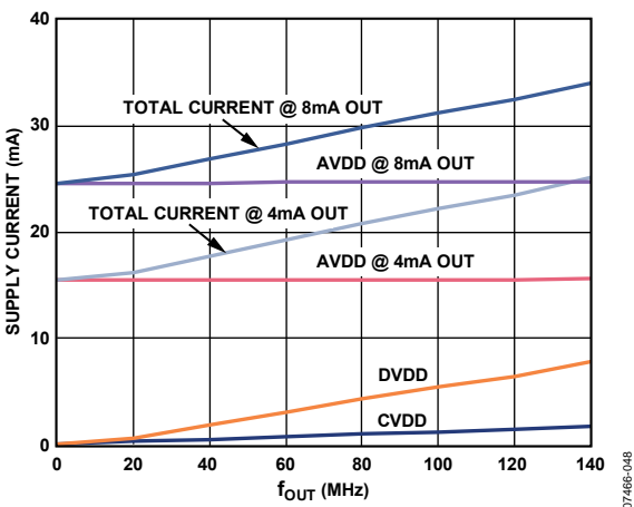
Figure 74. Supply Current vs. f_{OUT}
