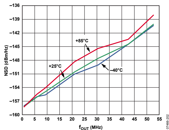
Figure 65. NSD at 8 mA, 3.3 V
