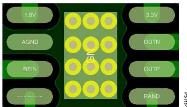
Figure 13. Evaluation Board Layout for the ADL5725 Package
