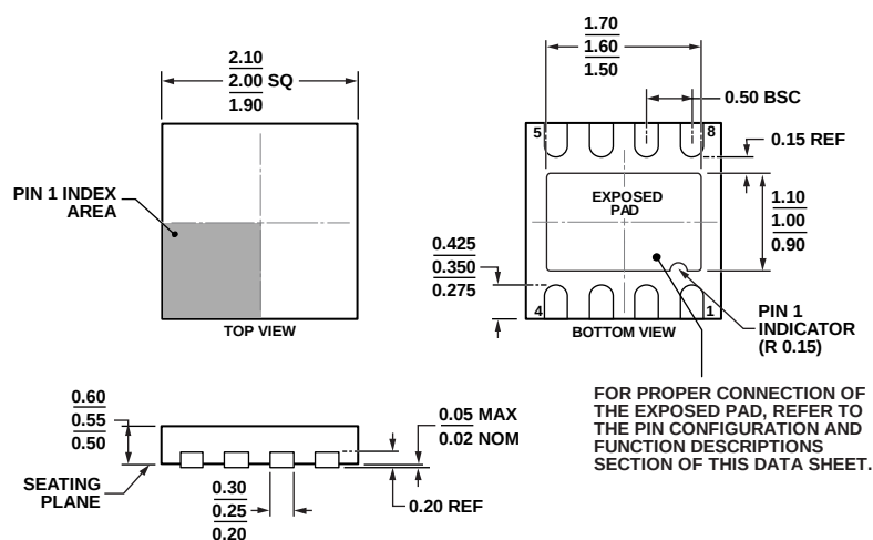
Figure 21. 8-Lead Lead Frame Chip Scale Package [LFCSP] 2.00 mm × 2.00 mm Body, and 0.55 mm Package Height (CP-8-10)
