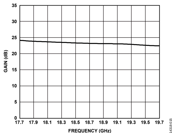
Figure 14. Gain vs. Frequency
