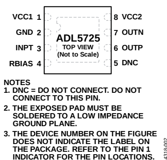
Figure 2. Pin Configuration
