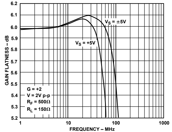
Figure 10. Gain Flatness—Large Signal
