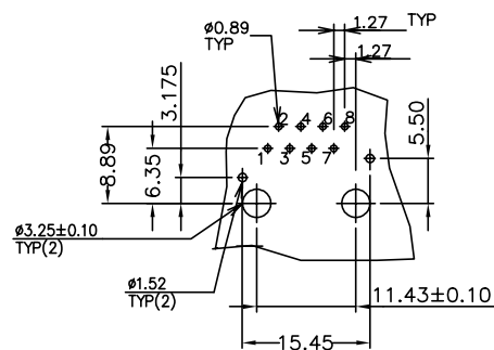
P.C.B. HOLE PATTERN VIEWED FROM TOP.
