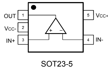
Figure 1. Pin connections (top view)
