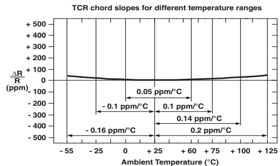
FIGURE 1 - TYPICAL RESISTANCE / TEMPERATURE CURVE (Z-FOIL)
