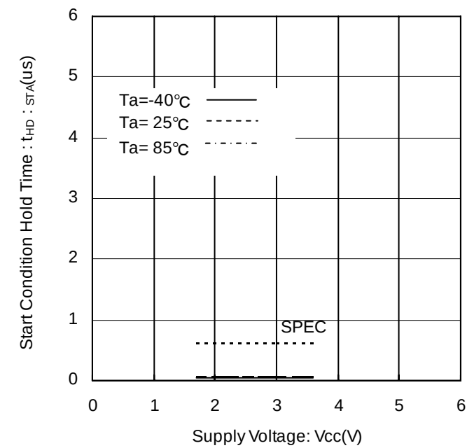
Figure 15. Start Condition Hold Time vs Supply Voltage
