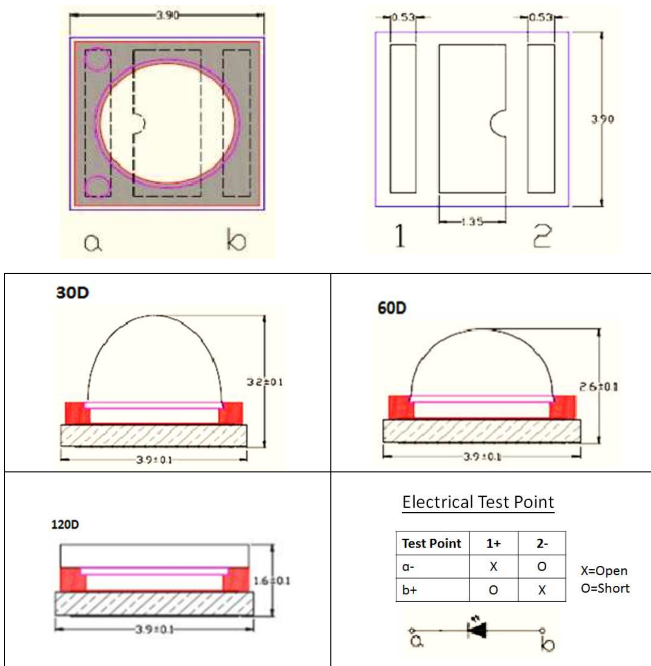
Figure 2. IN-C39ATKU1 / IN-C39BTKU1 / IN-C39CTKU1 Package Dimension
