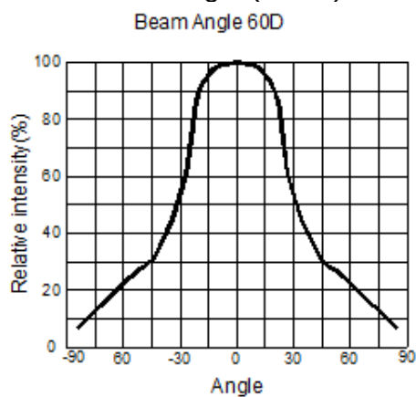
Beam Angle (2 \theta 1/2)
