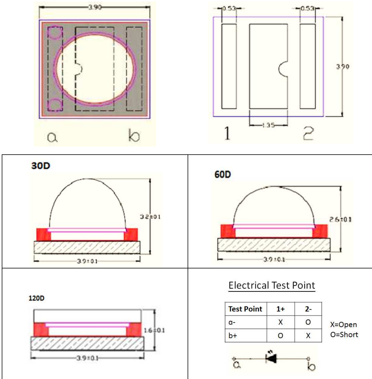
Figure 2. IN-C39ATKU1 / IN-C39BTKU1 / IN-C39CTKU1 Package Dimension
