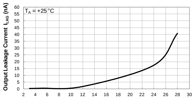
Supply Voltage (V) Output Leakage Current vs Supply Voltage
