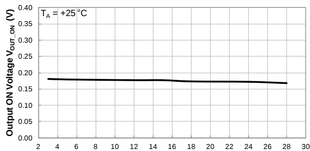
Supply Voltage (V) Output ON Voltage vs Supply Voltage
