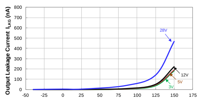
Temperature ( ^\circ\text{C} ) Output Leakage Current vs Temperature
