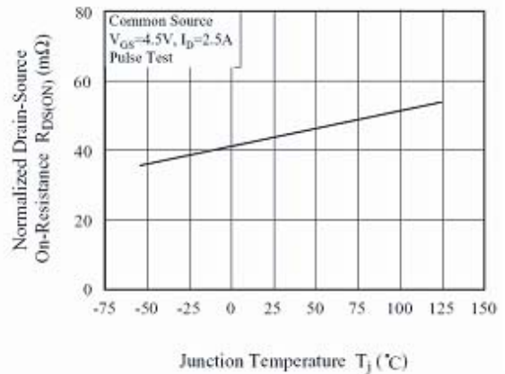
Fig4. R_{DS(on)} - T_J
