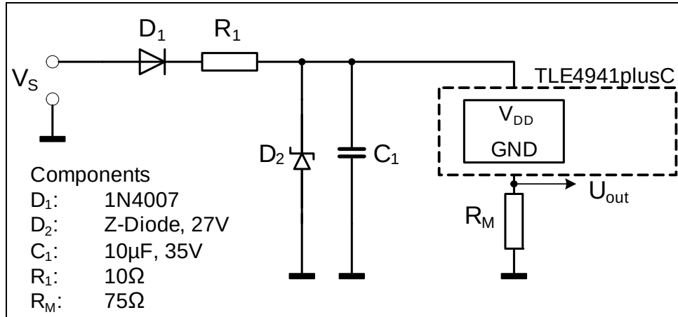
Figure 3-4 Application Circuit
