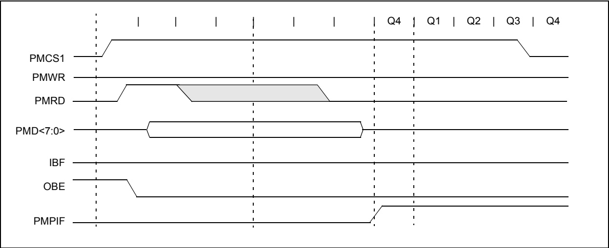
FIGURE 12-4: PARALLEL SLAVE PORT READ WAVEFORMS
