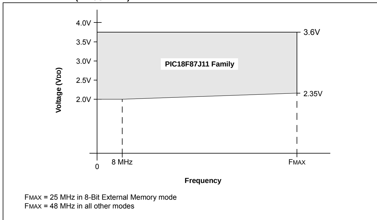
FIGURE 28-1: PIC18F87J11 FAMILY VOLTAGE-FREQUENCY GRAPH, REGULATOR ENABLED (INDUSTRIAL)
