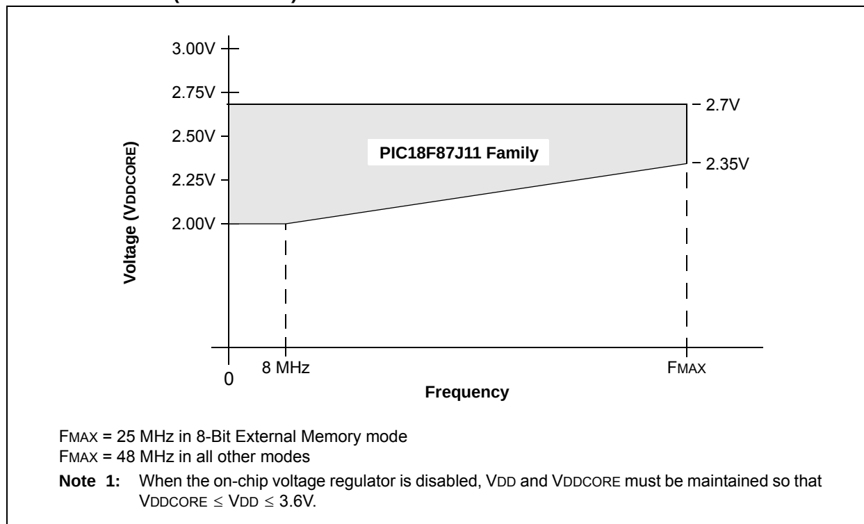
FIGURE 28-2: PIC18F87J11 FAMILY VOLTAGE-FREQUENCY GRAPH, REGULATOR DISABLED (INDUSTRIAL) 0
