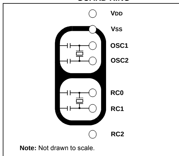
FIGURE 14-4: OSCILLATOR CIRCUIT WITH GROUNDED GUARD RING
