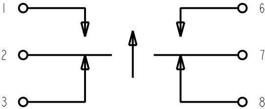
SCHEMATIC 2-C
