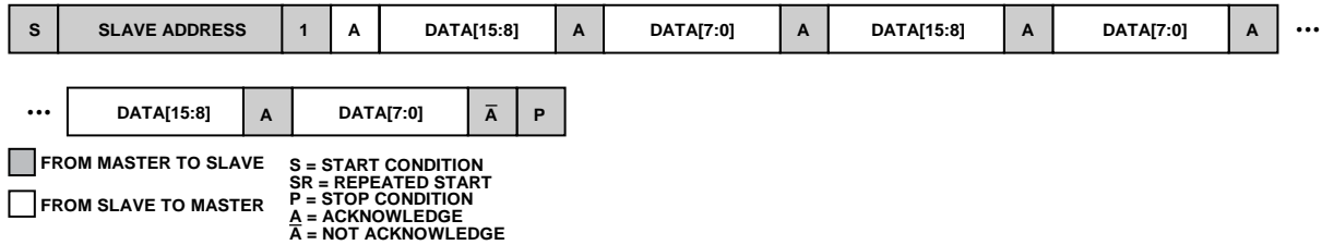
Figure 27. Reading Three Lots of Two Bytes of Data from the Conversion Result Register
