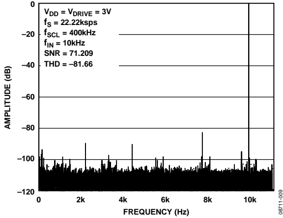
Figure 4. Typical FFT
