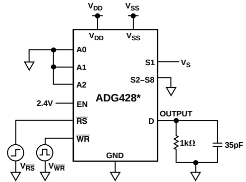
Test Circuit 8. Write Turn-On Time, t_{ON} (\overline{WR})
