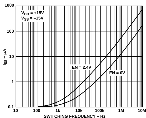
Figure 10. Negative Supply Current vs. Switching Frequency
