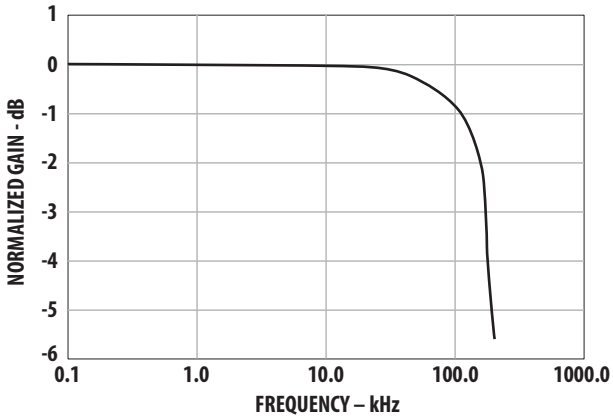
Figure 14. Bandwidth.
