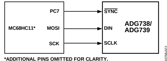
Figure 29. MC68HC11 Interface to ADG738/ADG739
