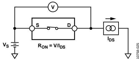
Figure 19. On Resistance
